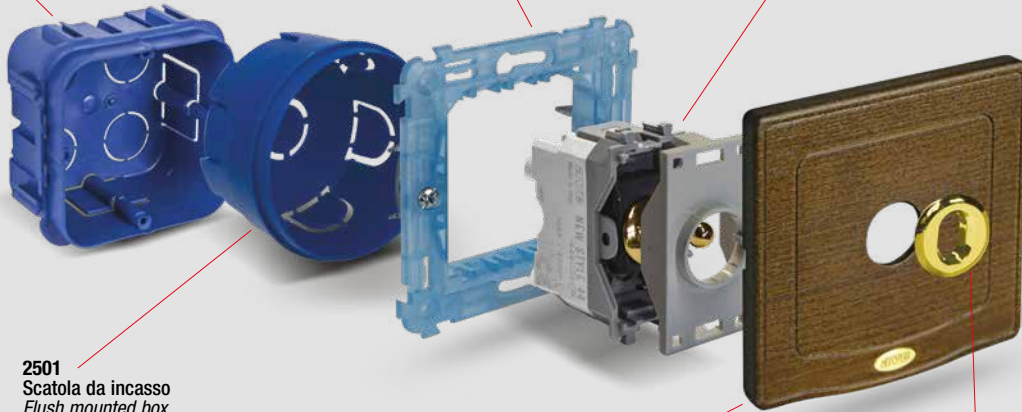
44PVNT21... (Vetro Glass) 44PANT21... (Alluminio Aluminium) 44PLET90... (Legno Wood) Placche NEW STYLE e ENGLAND STYLE NEW STYLE and ENGLAND STYLE front plates
