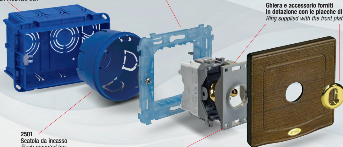
Comandi a levetta NEW STYLE e ENGLAND STYLE NEW STYLE and ENGLAND STYLE toggle controls
