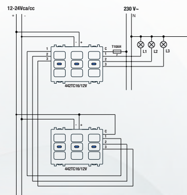
Comando luci da due 442TC16/12V Light control by two pcs 442TC16/12V
