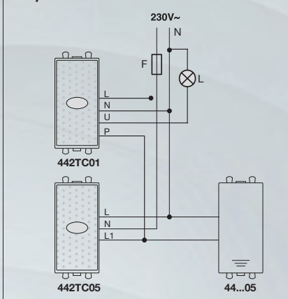
L: carico L: load F: fusibile F 1,6A H F: fuse F 1,6A H
